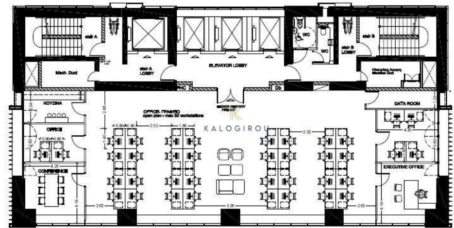
OFFICE FLOOR PLAN
