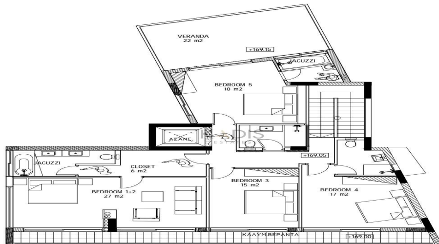
FIRST FLOOR Total area 185 sq.m.
