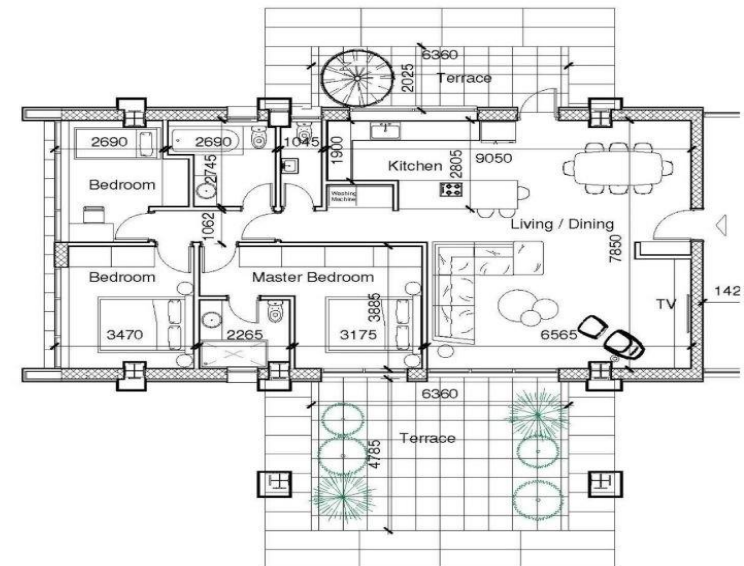
PLAN 2 ND FLOOR
