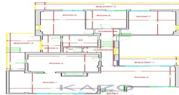
PLAN ( GROUND FLOOR ) = 200 M2
