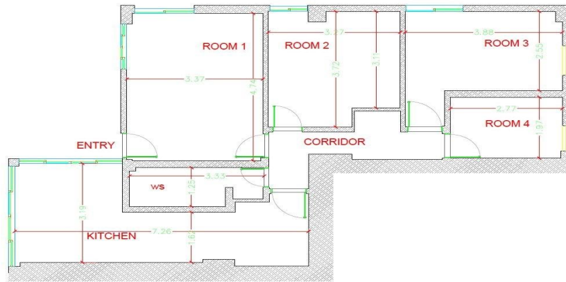
PLAN ( BASEMENT FLOOR ) = 80 M2
