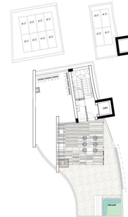
Villa 2 - Roof Garden Plan
