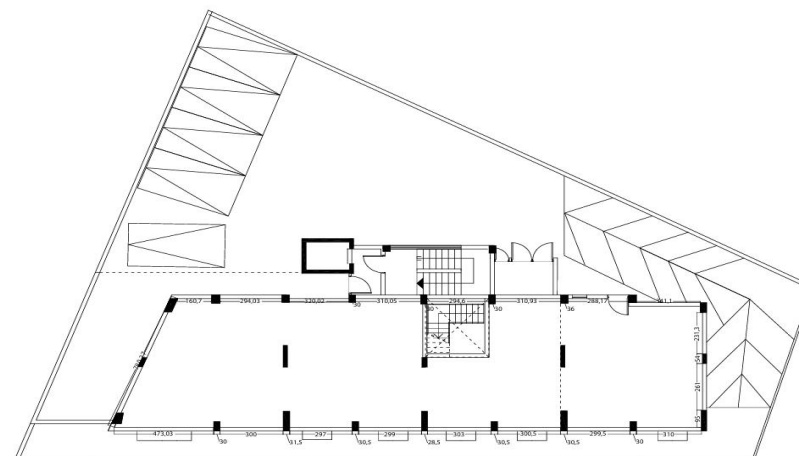
BASEMENT FLOOR TOTAL AREA: 203,25 m2
