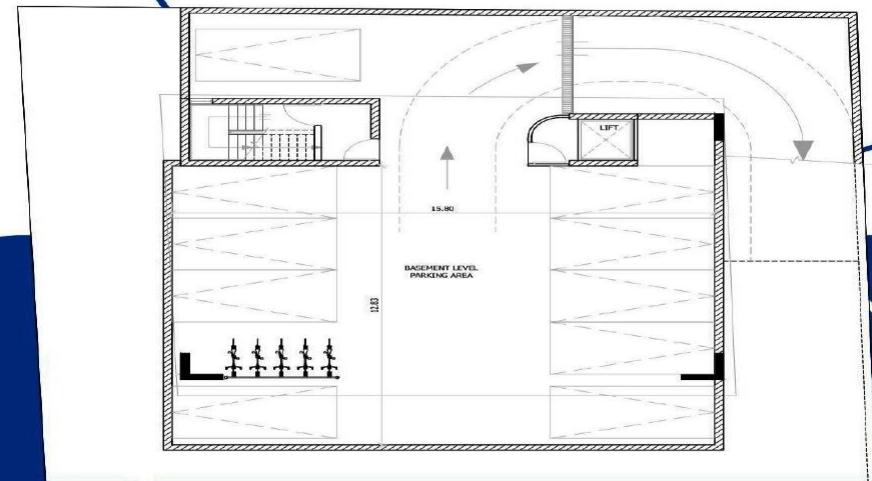
BASEMENT PLAN
