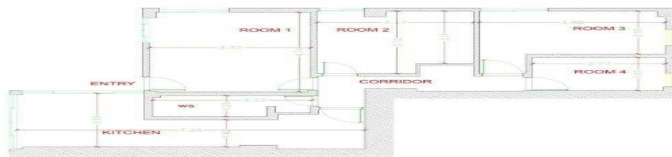
PLAN ( BASEMENT FLOOR ) = 80 M2
