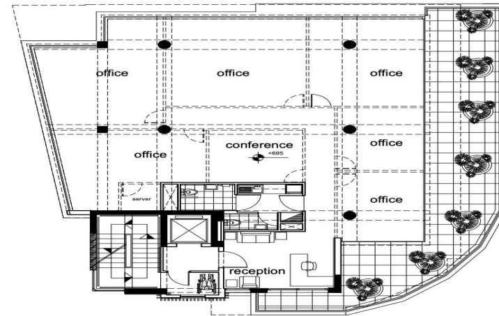
1st floor - office
