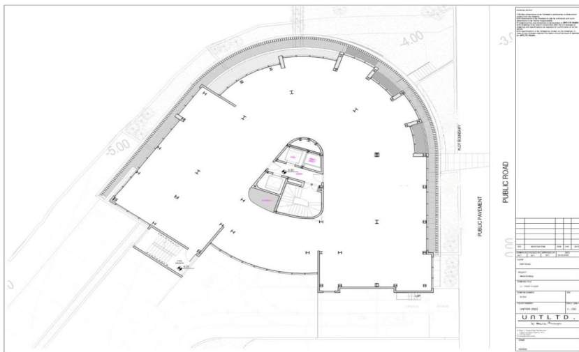
Level 2 Floor Plan
