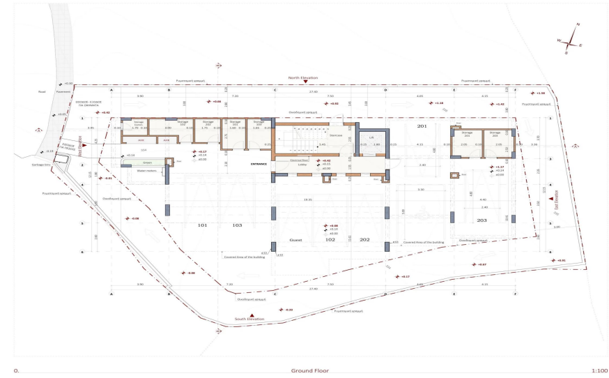
0. Ground Floor 1:100
