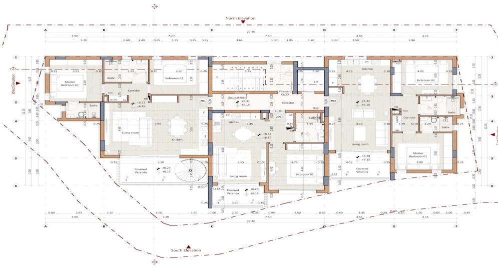
2. 2nd Floor 1:100
