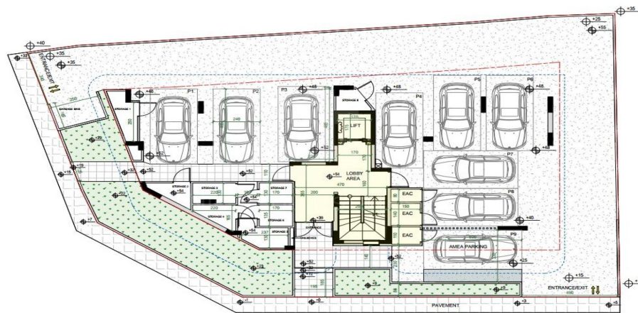
GROUND FLOOR PLAN SCALE 1:200
