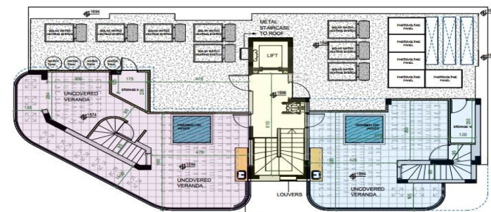
ROOF GARDEN FLOOR PLAN SCALE 1:200
