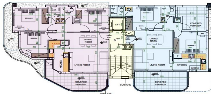
SECOND FLOOR PLAN SCALE 1:200
