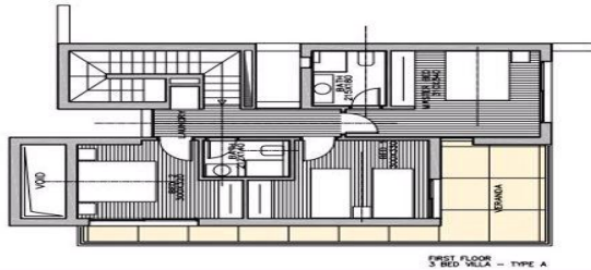
FIRST FLOOR 3 BED VILLA - TYPE A
