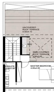
ROOF TERRACE
