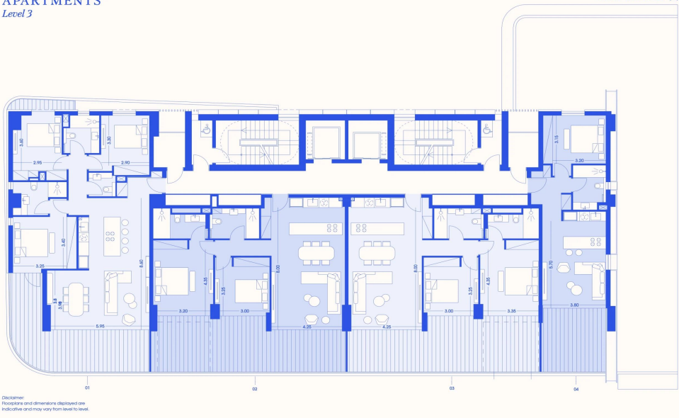
APARTMENTS Level 3
