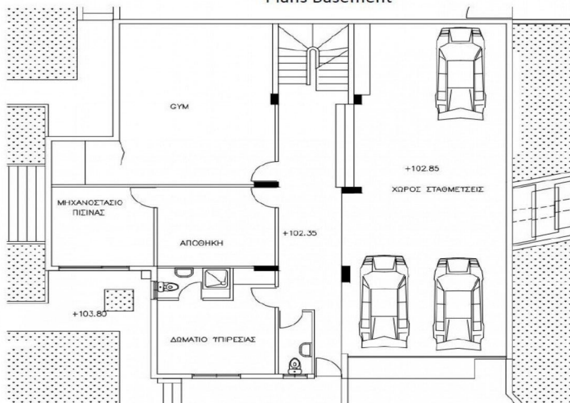
Plans Basement
