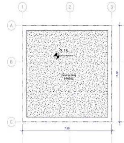
ROOF PLAN
