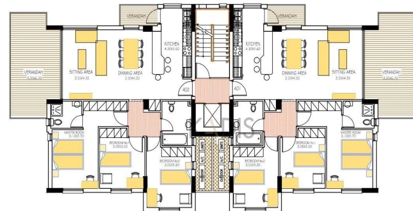
4th FLOOR PLAN
