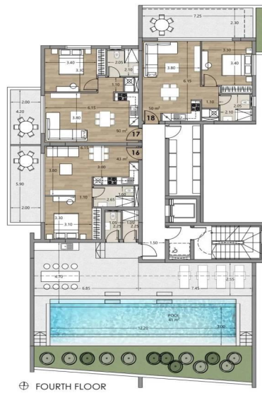
FOURTH FLOOR
