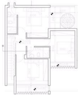
UPPER FLOOR
