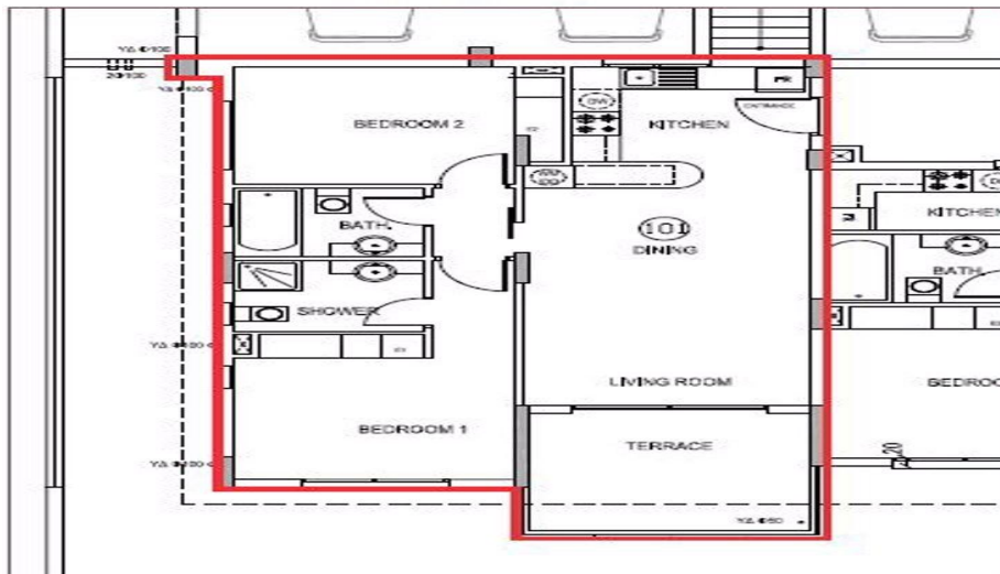
APARTMENT PLAN
