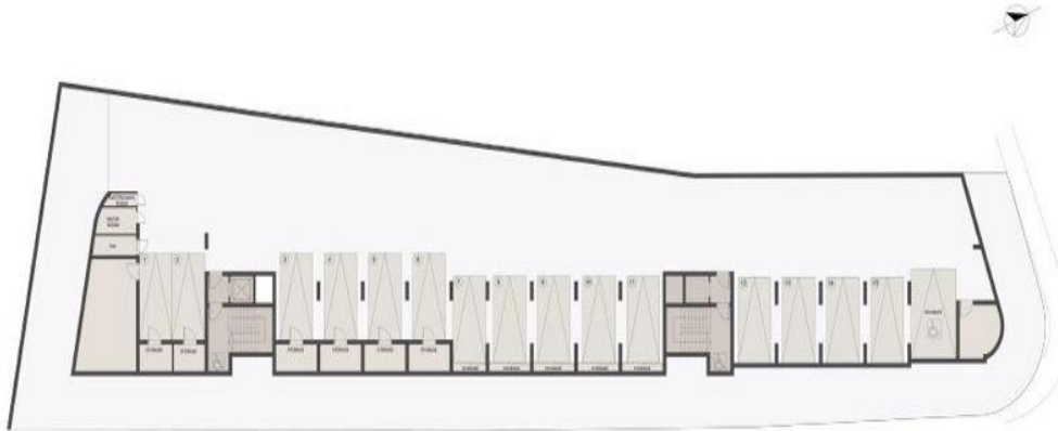
BLOCK A & B - FIRST FLOOR PLAN
