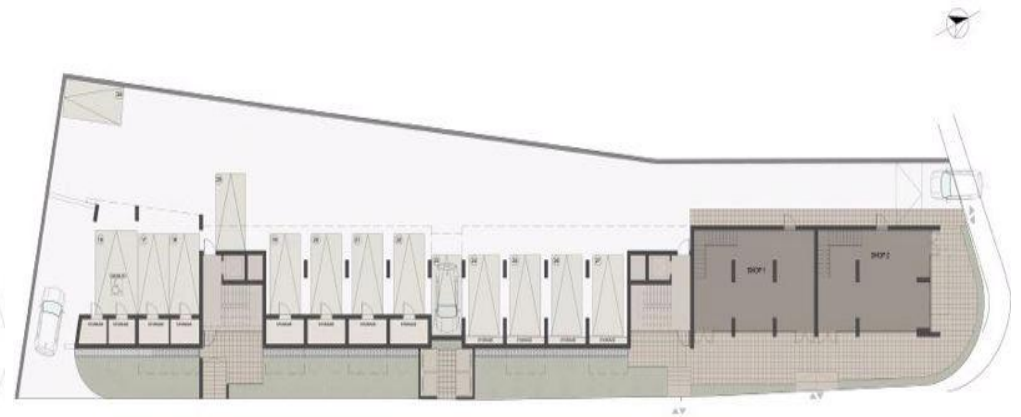
BLOCK A & B - GROUND FLOOR PLAN
