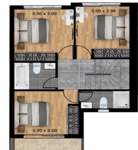
Block C - Unit # 34 Internal Area # 105 SQM Covered Veranda # 4 SQM Plot Area # 107 SQM
