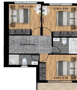
Block C - Unit # 33 Internal Area # 105 SQM Covered Veranda # 4 SQM Plot Area # 106 SQM
