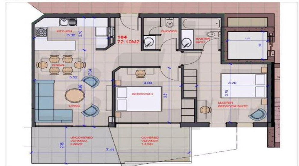
PRELIMINARY APARTMENT PLAN
