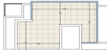
Roof Plan
