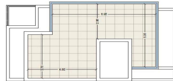
Roof Plan
