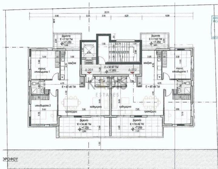
SECOND TO FOURTH Floor Plan
