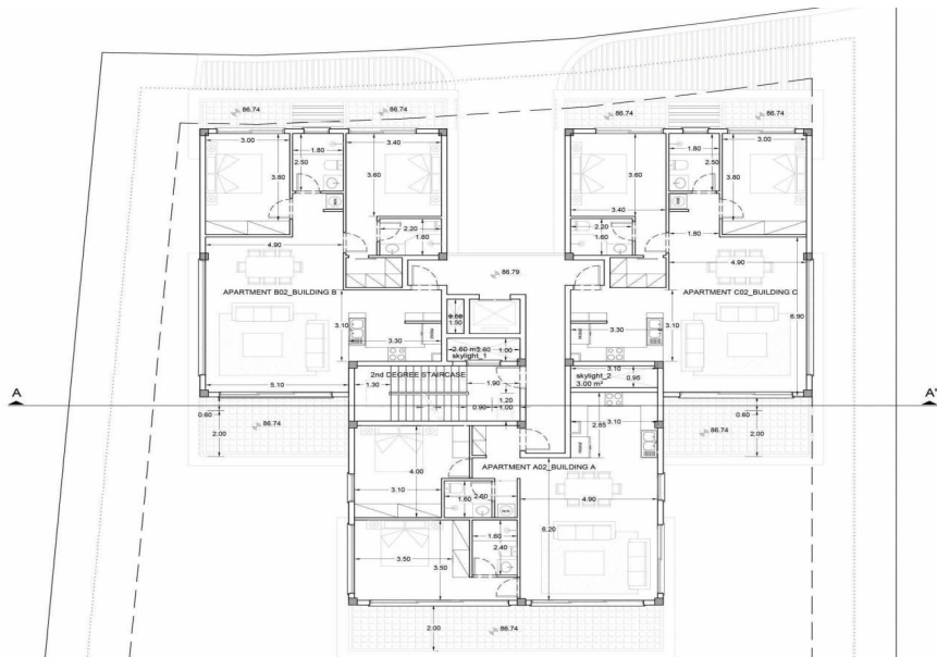
3 Bedroom Plan
