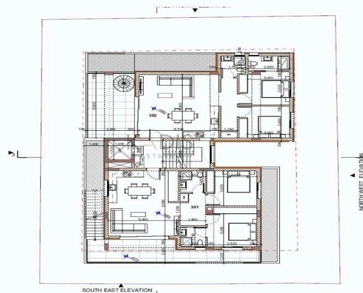
3rd Floor
