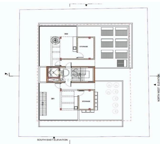
Roof Garden
