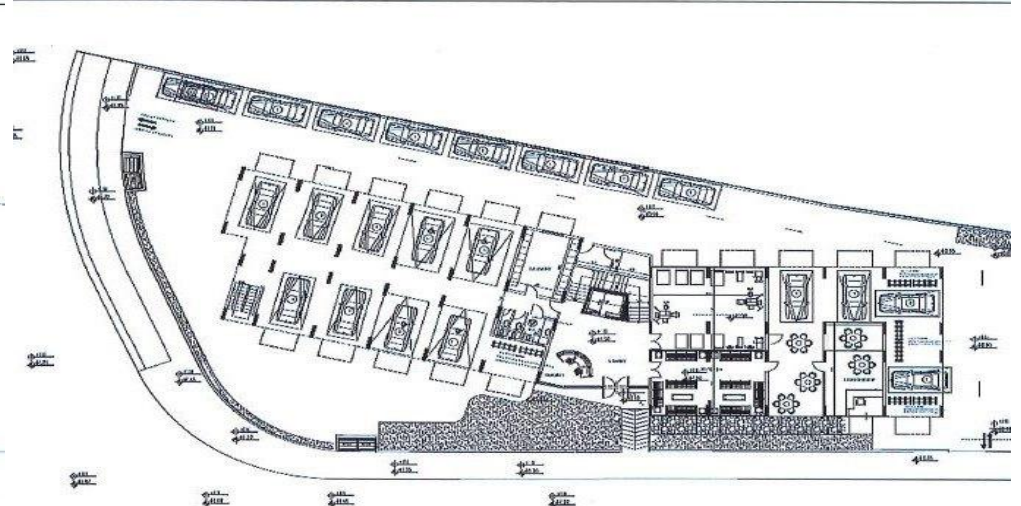
GROUND FLOOR LAYOUT
