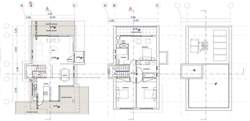
FLOOR PLANS
