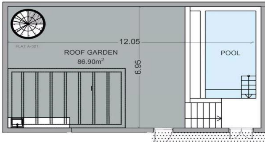
BLOCK A - ROOF PLAN APARTMENT 301
