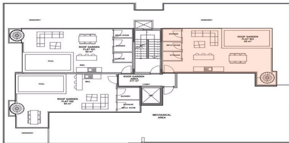
6. Roof Garden 1:100
