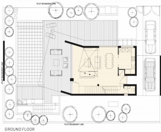
3 BEDROOM VILLA
