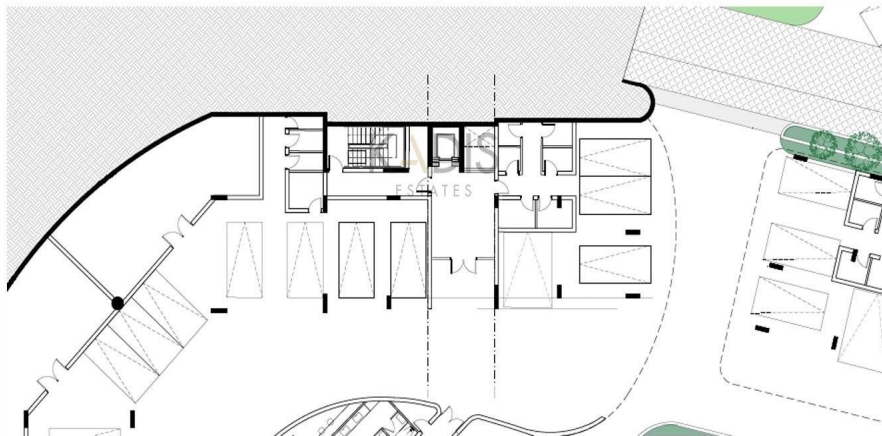
BUILDING C LOWER GROUND FLOOR
