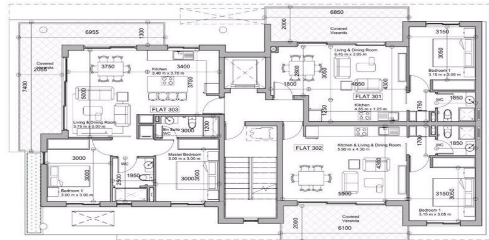
Drawings - 3 rd Floor
