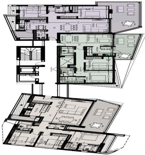
TYPICAL FLOOR PLAN FLOORS 2,3
