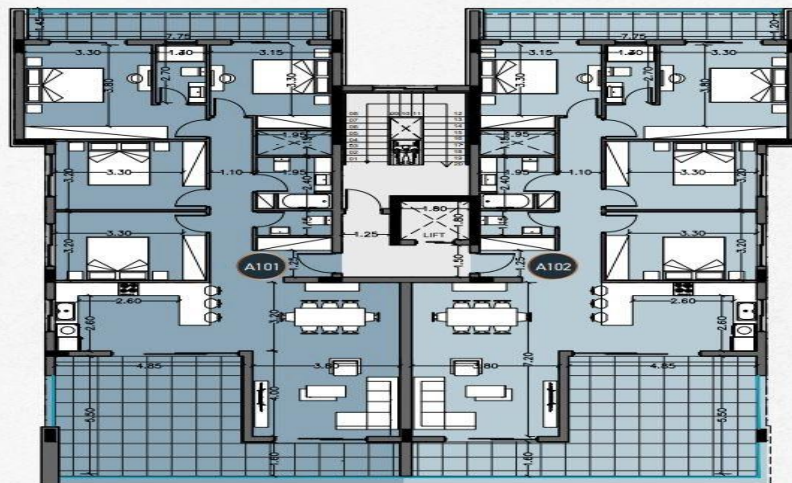
1st Floor
