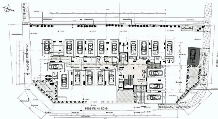
Parking Plan
