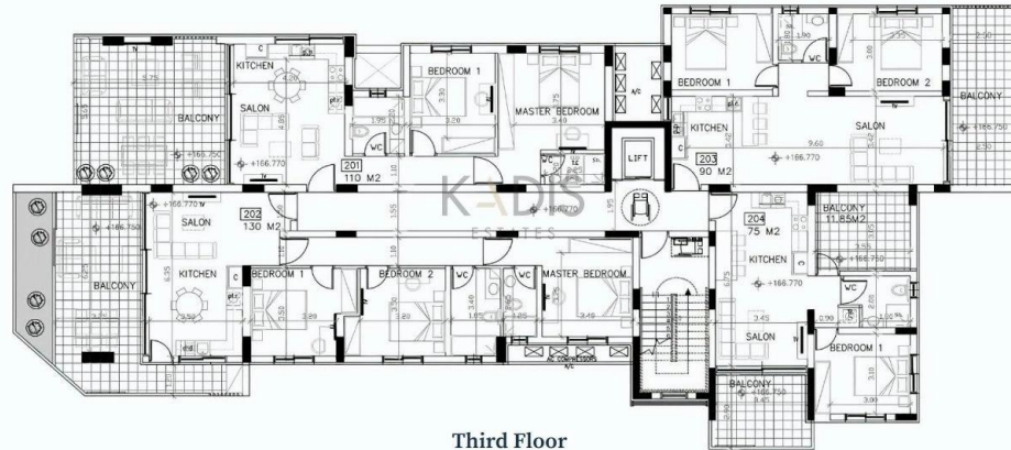
Third Floor
