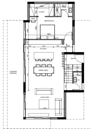
GROUND FLOOR 1 : 100
