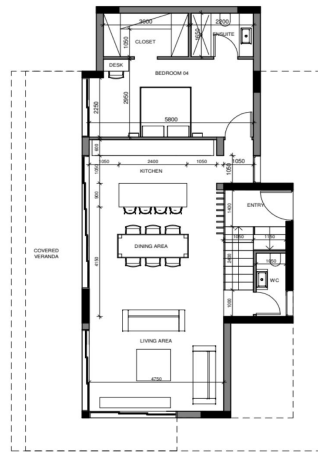
GROUND FLOOR 1 : 100
