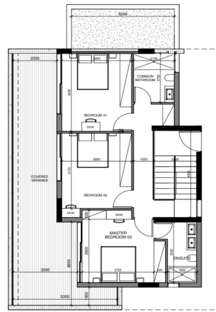
FIRST FLOOR 1 : 100
