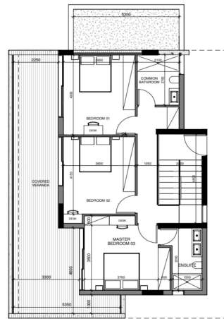
FIRST FLOOR 1 : 100
