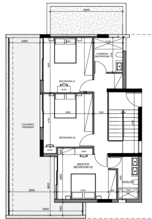
FIRST FLOOR 1 : 100
