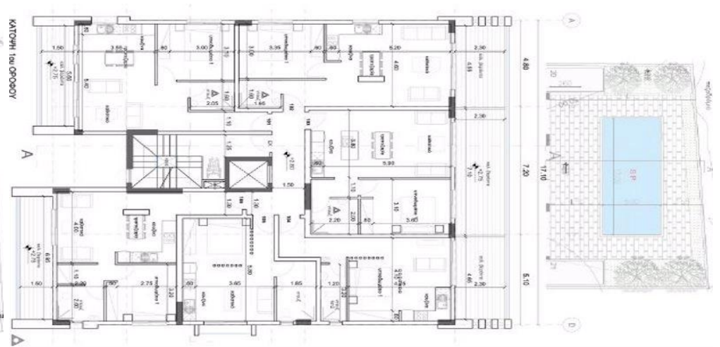
FLOOR PLAN 1st floor
