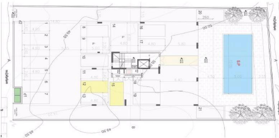
SITE PLAN
