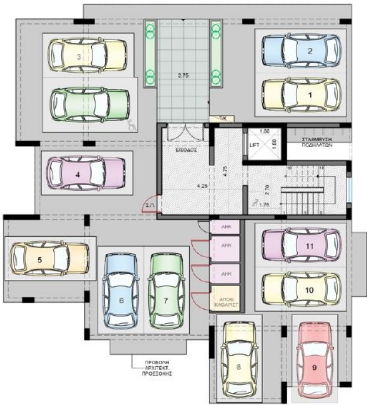
SOUTH GROUND FLOOR PLAN
