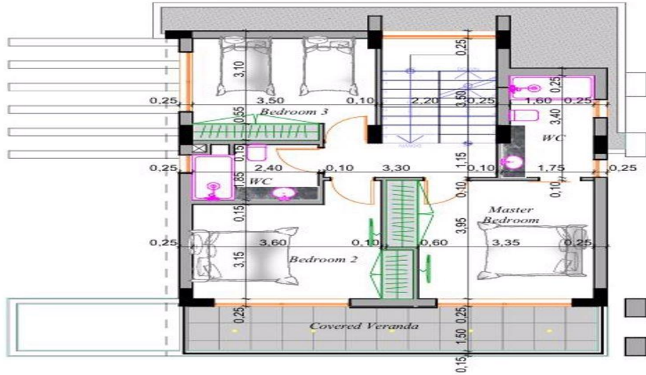
1. 1st Floor 1:100
