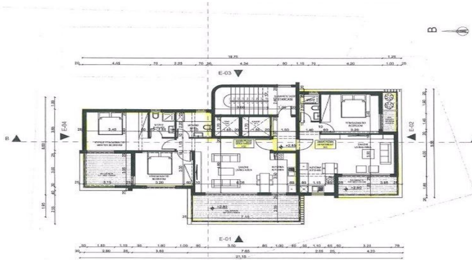
ΚΑΤΩΦΗ 1ου ΟΡΟΦΟΥ FIRST FLOOR PLAN
