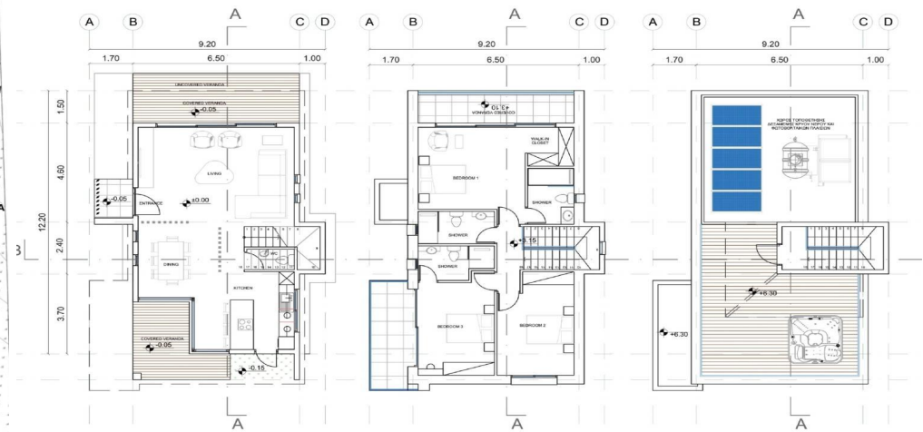
FLOOR PLAN
