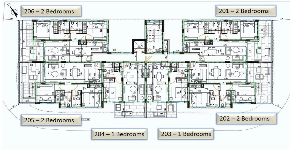
2nd floor plans - Provisional
