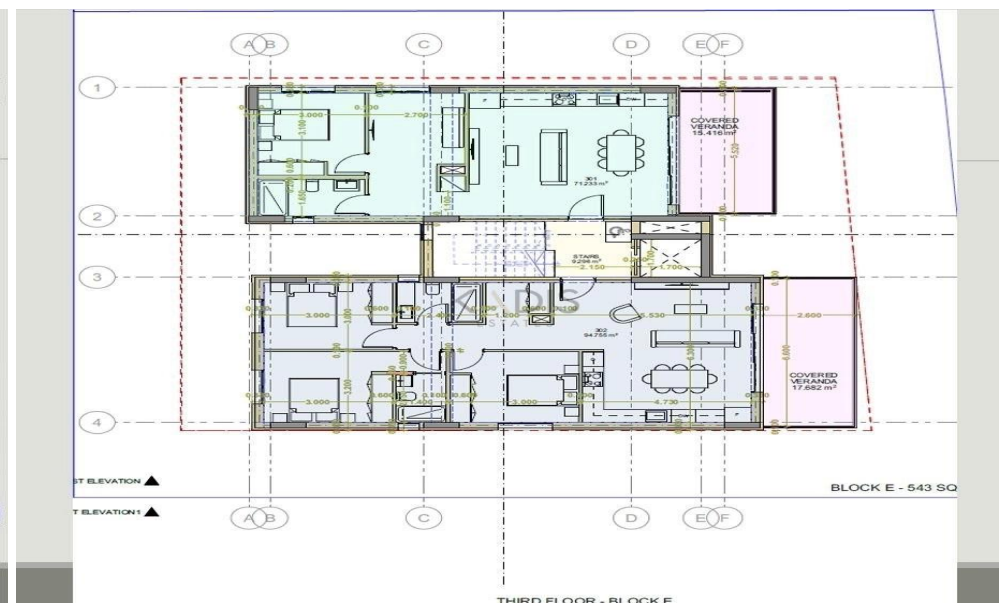
THIRD FLOOR - BLOCK E
