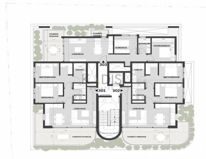
3rd FLOOR
