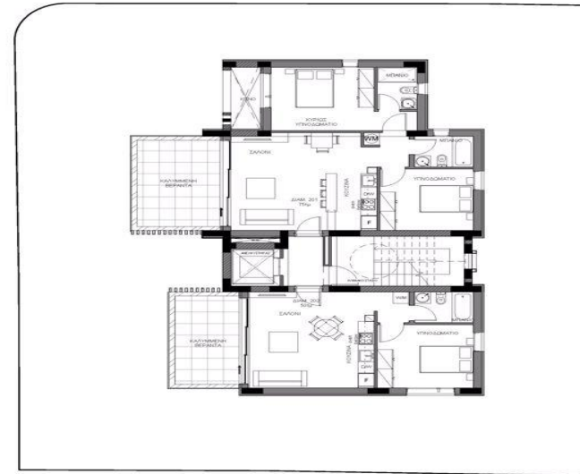
SECOND FLOOR
